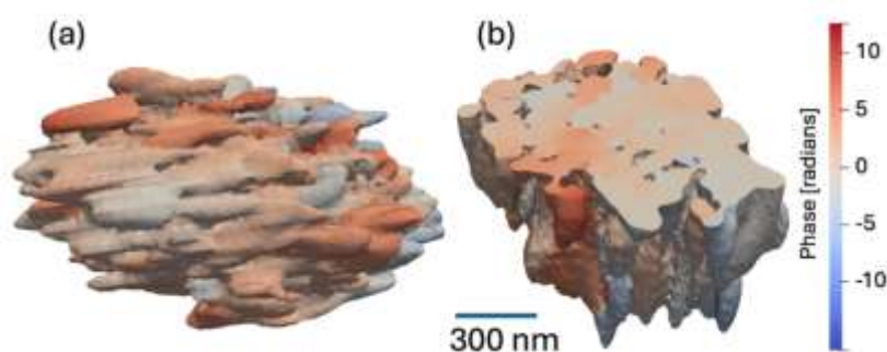
(a) External surface of a 1600 nm sized \text{Li}_3\text{Ti}_2(\text{PO}_4)_3 crystal measured by BCDI on a 110 Bragg peak. The cigar shaped domains are oriented along the hexagonal crystal's c -axis, horizontally on the page. (b) Cross section perpendicular to the c -axis showing a network of phase domains. Ion diffusion is expected to take place along the domain boundaries.
