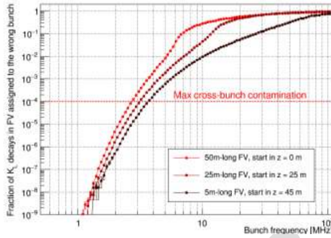
Figure 3.21: Fraction of K_L decays in fiducial volume assigned to the wrong bunch, as a function of bunch frequency in MHz, for three different definitions of fiducial volume.
