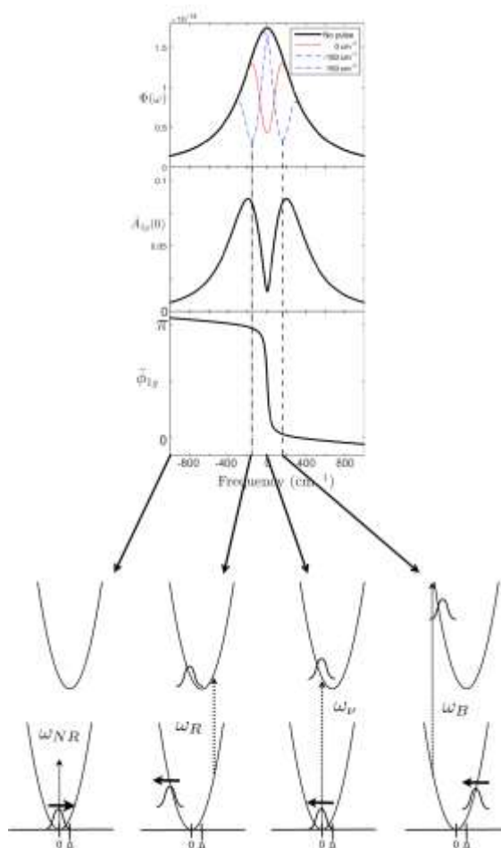
Figure 7.16: Illustration of the lineshape theory treatment of ground and excited state vibrational coherence calculation using additional wavepacket representations.
