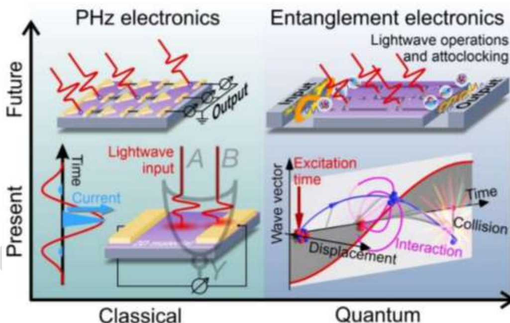
Figure 5.10: The emerging field of lightwave electronics
