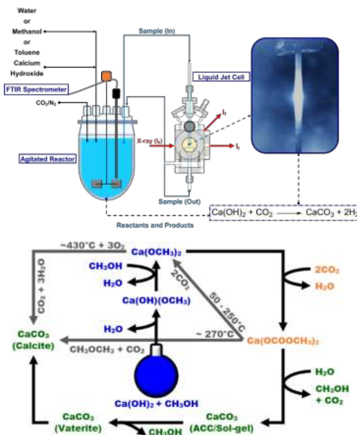
Figure 8.2: (Top) Liquid-jet time-resolved XAS operando probing of the multiphase-multicomponent synthesis of surfactant-stabilised \text{CaCO}_3 detergent particles.
