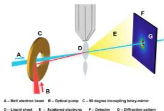
Figure A1.4: Schematic representation of the liquid-phase MeV UED experimental setup
