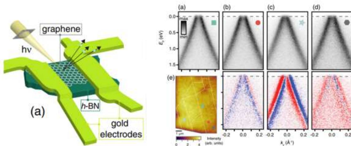
Left: Graphene on h-BN with gold source-drain electrodes to inject 'transport current' at THz frequencies. Right: Intensity of the Dirac cone spectra taken in different locations of the device, as given by the corresponding markers in (e) [reproduced with permission from 3].
