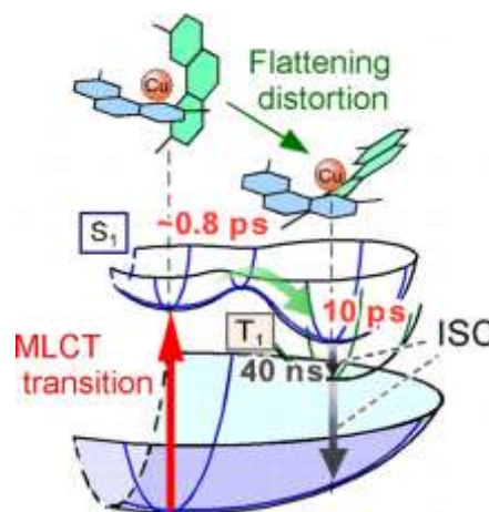
Figure 6.7: Light-triggered distortion in a Cu-complex. Ultrafast nuclear, spin and electronic, dynamics are convolved. 37
