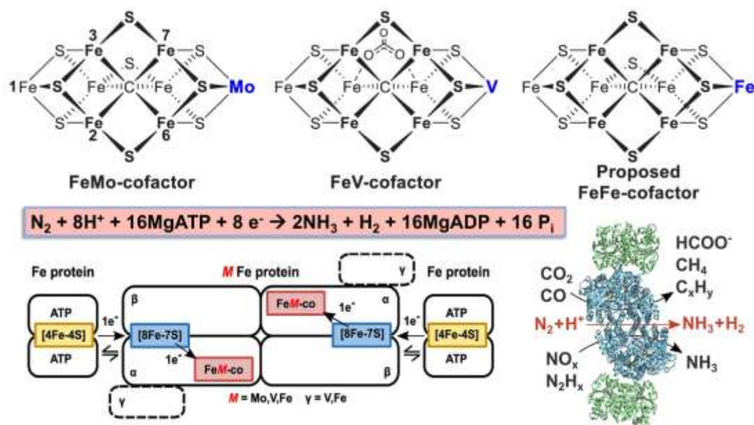
Figure 8.13: (Bottom, left) Schematic of nitrogenase structures showing the electron delivery Fe protein component and the catalytic MFe protein component (M = Mo, V, Fe). (Bottom, right) Overall structure of Fe protein - MoFe protein complex and reactions catalysed. (Centre) The nitrogenase reaction is catalysed by the metal FeM-co centres (top) that incorporate similar but distinct clusters from various microbes.
