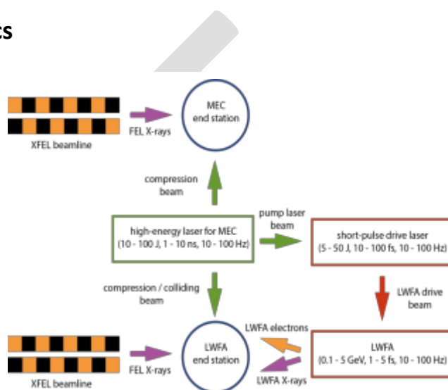
Figure 4.3: Schematic diagram illustrating how auxiliary lasers at an XFEL could drive a LWFA
