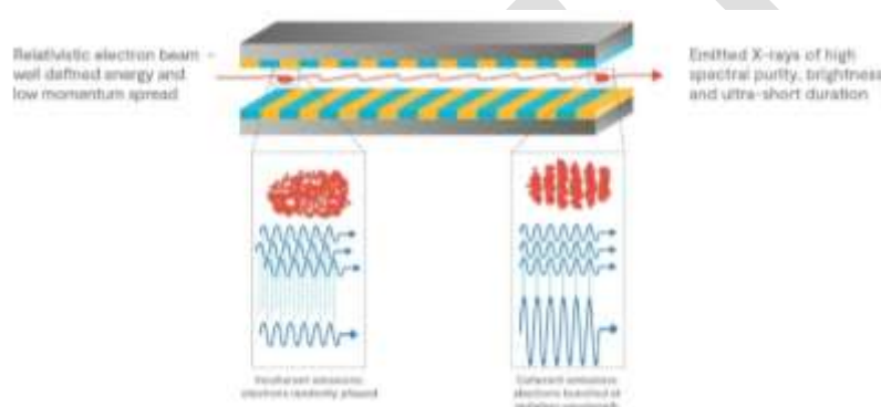
Figure 2.1: Principle of operation of a SASE X-ray free electron laser
