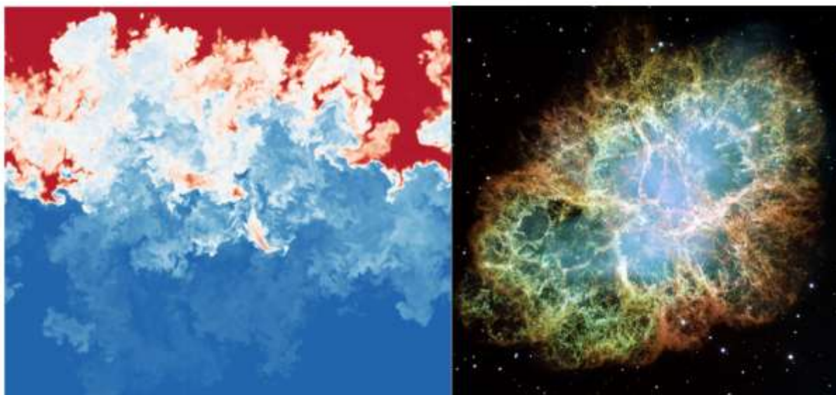
Left: Simulation of a turbulent fluid mixing during shock-compression of an imperfect interface from [1].
