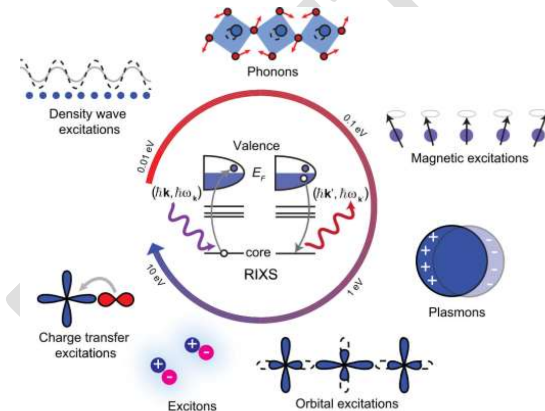
Figure 5.1: The resonant scattering process, shown in the centre, involves the resonant absorption of an X-ray photon, creating an intermediate state with a core hole and a valence excitation, before the hole is filled via the emission of another X-ray photon. Measuring the momentum-change of the scattering, in a so-called resonant diffraction experiment, can probe electronic order parameters such as magnetic order. By measuring the energy and momentum change of the X rays in a resonant inelastic X-ray scattering (RIXS) experiment, one can infer the properties of the excitations created in the material. The many different types of excitation that RIXS can probe are shown around the outside. 6
